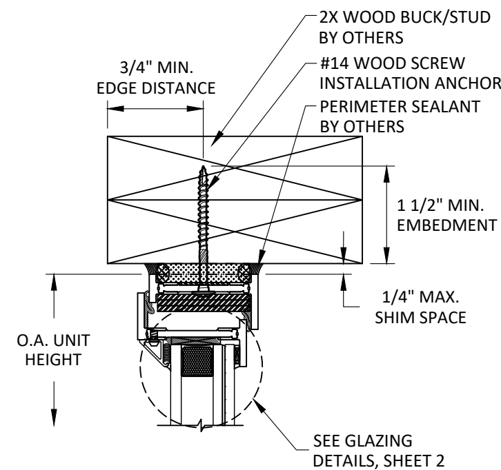
A 11 VERTICAL SECTION HEAD - 2X WOOD BUCK THROUGH FRAME INSTALLATION SHORT LEG FRAME
