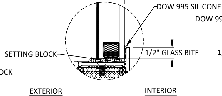
GLAZING DETAIL 2
