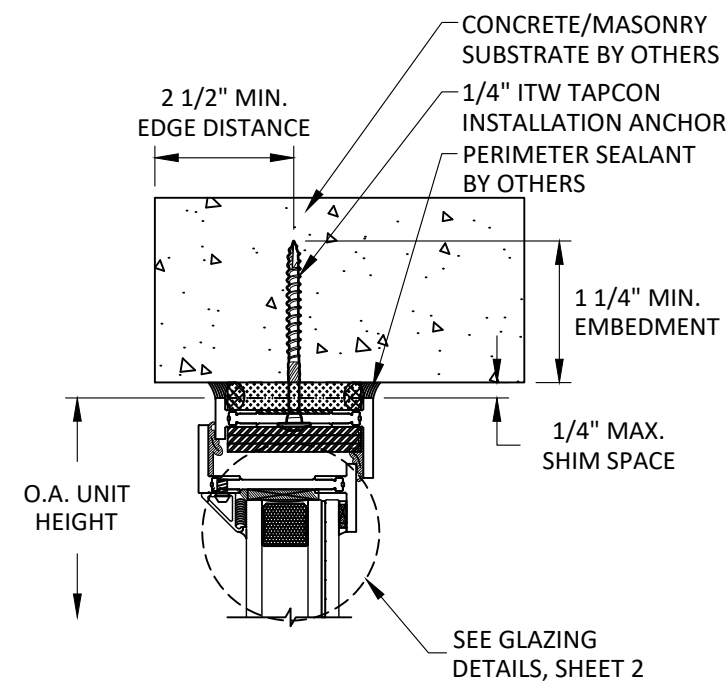
B 11 VERTICAL SECTION HEAD - CONCRETE/MASONRY THROUGH FRAME INSTALLATION SHORT LEG FRAME
