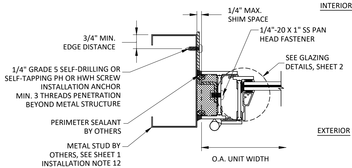
A HORIZONTAL SECTION 10 JAMB- METAL STUD STRAP INSTALLATION LONG LEG FRAME
