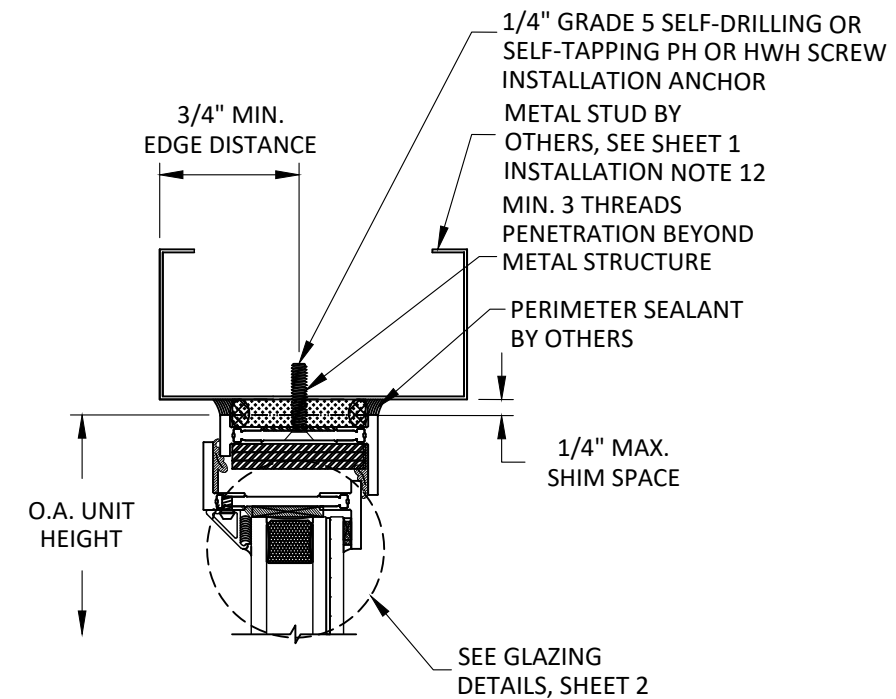
C 11 VERTICAL SECTION HEAD - METAL STUD THROUGH FRAME INSTALLATION SHORT LEG FRAME
