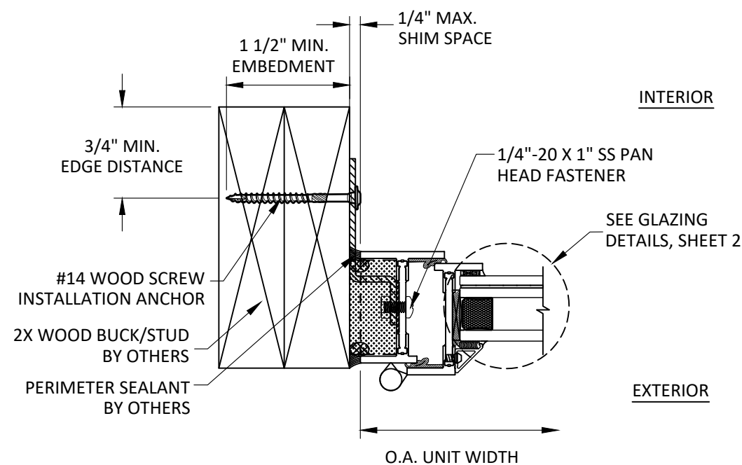
A 8 HORIZONTAL SECTION JAMB- 2X WOOD BUCK STRAP INSTALLATION LONG LEG FRAME
