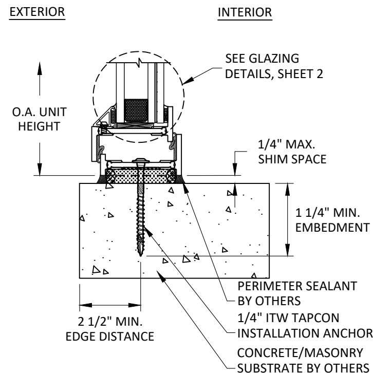
E 11 VERTICAL SECTION SILL - CONCRETE/MASONRY THROUGH FRAME INSTALLATION SHORT LEG FRAME
