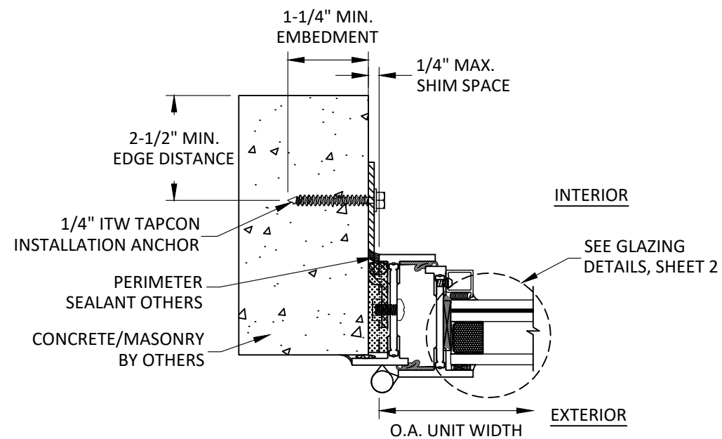
C 9 HORIZONTAL SECTION JAMB- CONCRETE/MASONRY FLANGE/STRAP INSTALLATION UNEQUAL LEG FRAME
