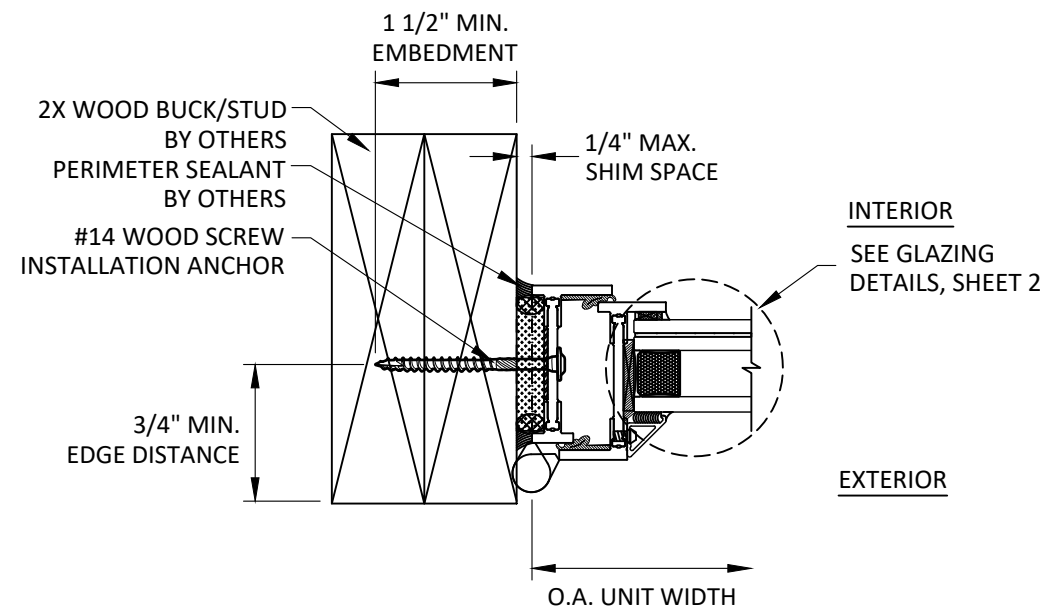
A HORIZONTAL SECTION 12 JAMB- 2X WOOD BUCK THROUGH FRAME INSTALLATION SHORT LEG FRAME
