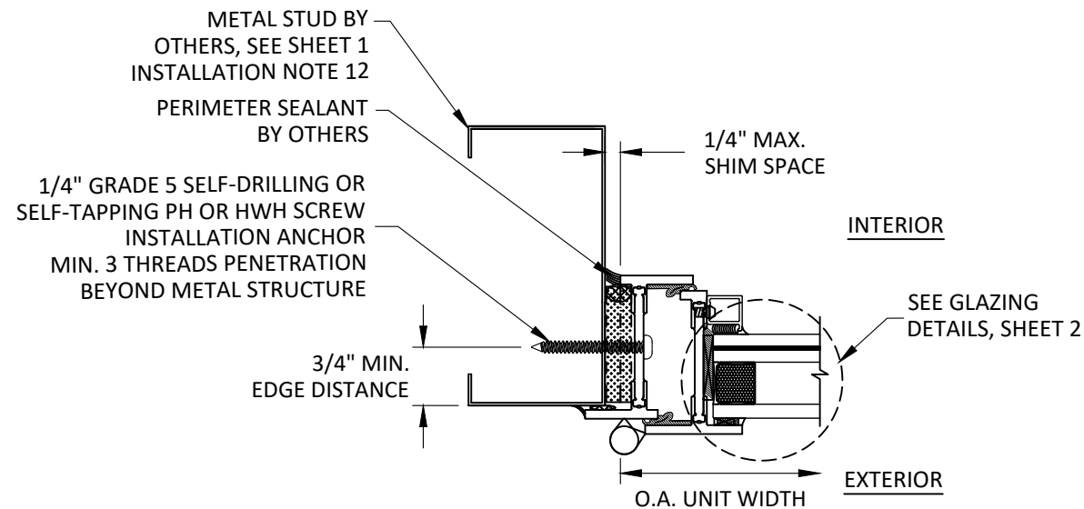
C HORIZONTAL SECTION 10 JAMB- METAL STUD FLANGE INSTALLATION UNEQUAL LEG FRAME
