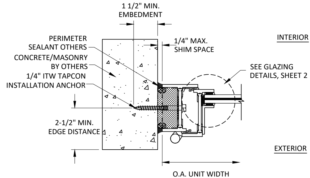
B 9 HORIZONTAL SECTION JAMB- CONCRETE/MASONRY THROUGH FRAME INSTALLATION LONG LEG FRAME
