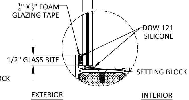
GLAZING DETAIL 4
