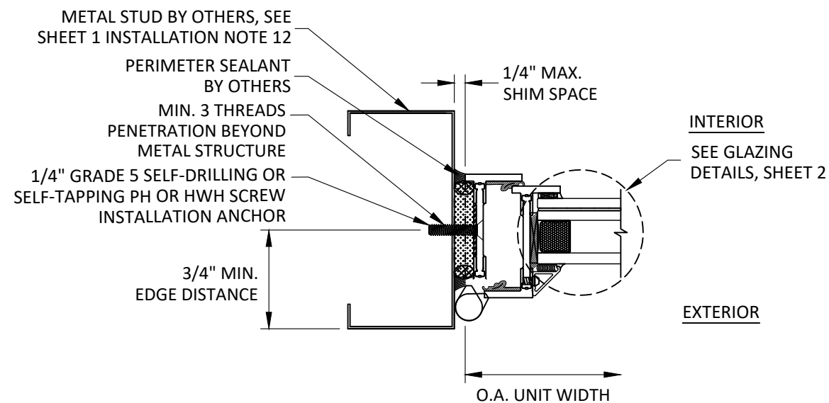
C HORIZONTAL SECTION 12 JAMB- METAL STUD THROUGH FRAME INSTALLATION SHORT LEG FRAME
