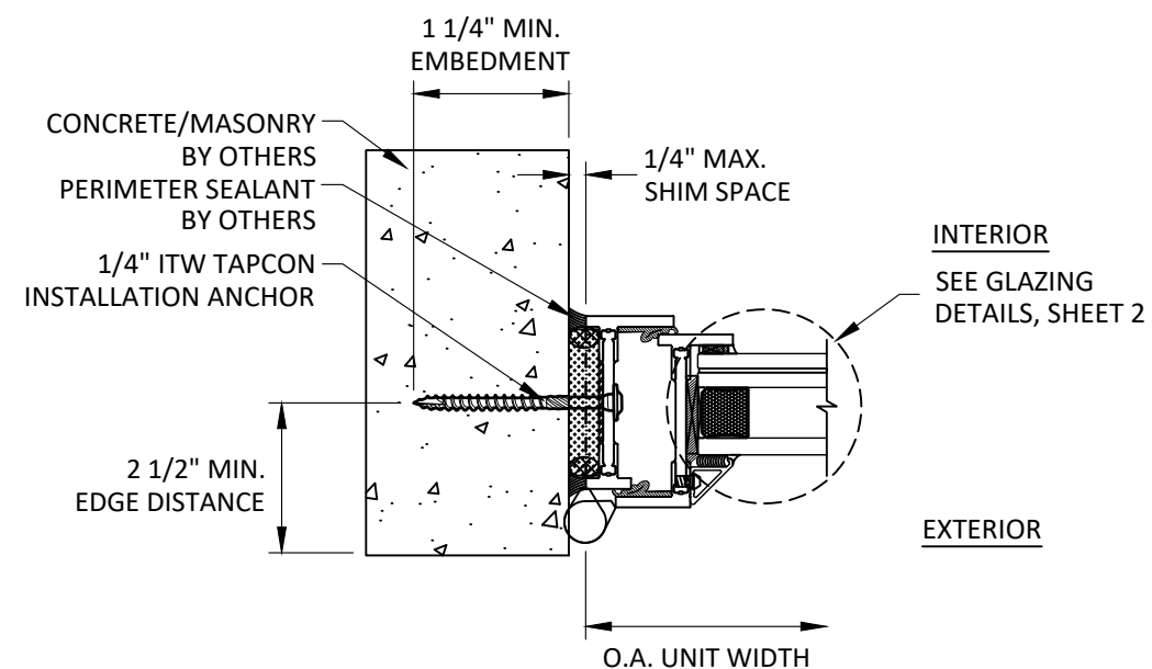
B HORIZONTAL SECTION 12 JAMB- CONCRETE/MASONRY THROUGH FRAME INSTALLATION SHORT LEG FRAME
