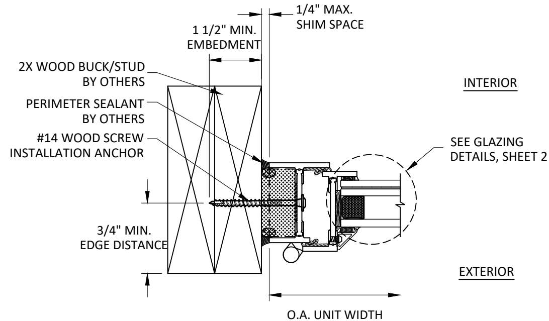
B 8 HORIZONTAL SECTION JAMB- 2X WOOD BUCK THROUGH FRAME INSTALLATION LONG LEG FRAME
