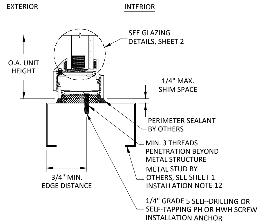
F 11 VERTICAL SECTION SILL - METAL STUD THROUGH FRAME INSTALLATION SHORT LEG FRAME
