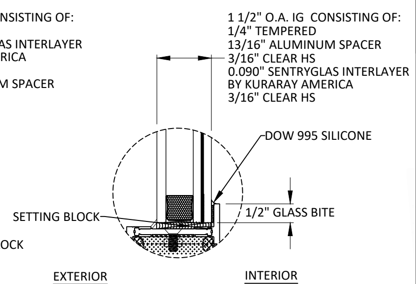
GLAZING DETAIL 8
