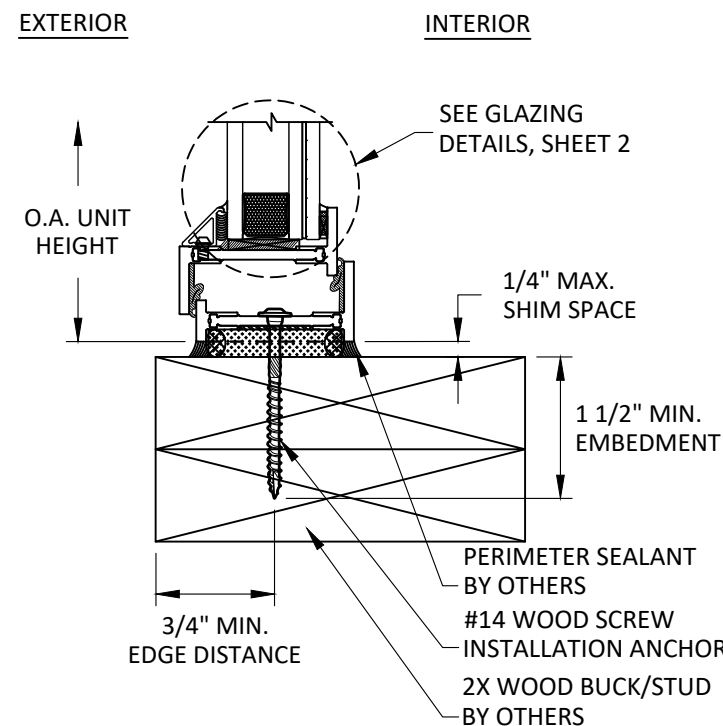
D 11 VERTICAL SECTION SILL - 2X WOOD BUCK THROUGH FRAME INSTALLATION SHORT LEG FRAME
