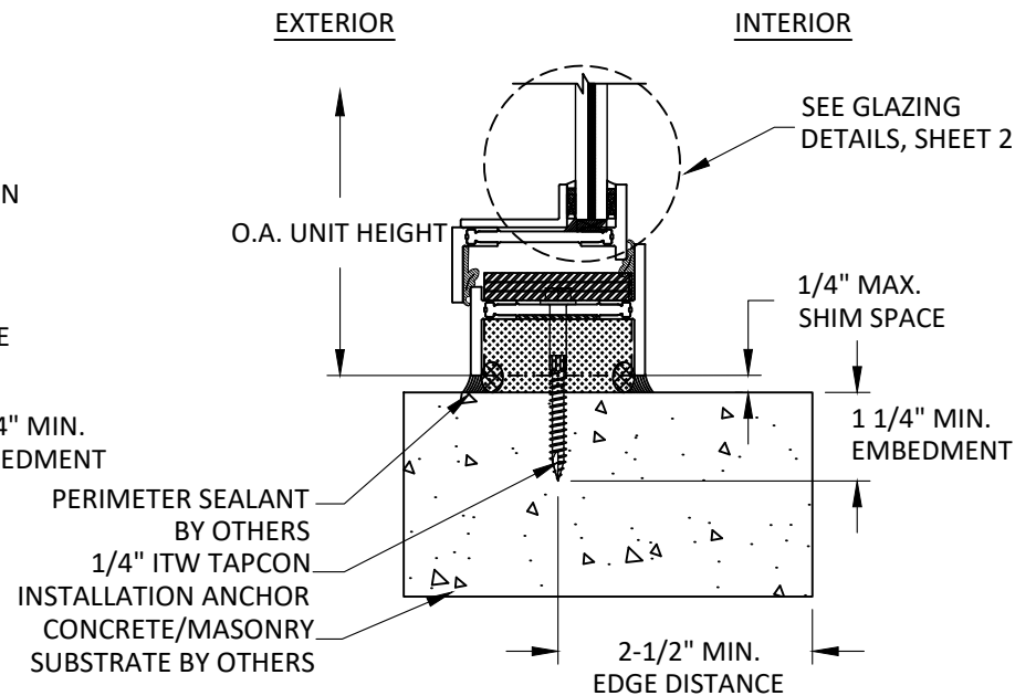
E 6 VERTICAL SECTION SILL - CONCRETE/MASONRY THROUGH FRAME INSTALLATION LONG LEG FRAME
