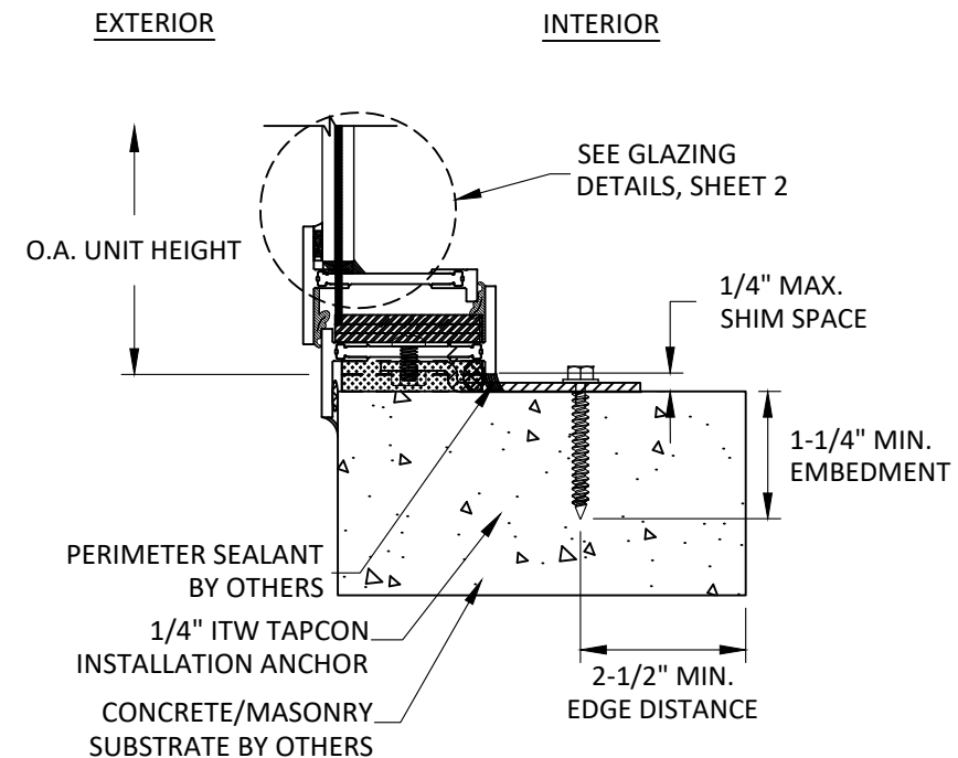
F 6 VERTICAL SECTION SILL - CONCRETE/MASONRY FLANGE/STRAP INSTALLATION UNEQUAL LEG FRAME
