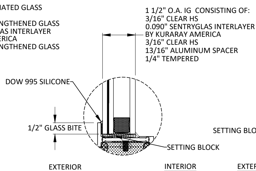
GLAZING DETAIL 7
