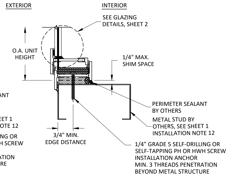
F 7 VERTICAL SECTION SILL - METAL STUD FLANGE INSTALLATION UNEQUAL LEG FRAME
