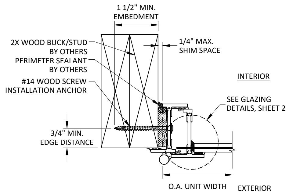
C 8 HORIZONTAL SECTION JAMB- 2X WOOD BUCK FLANGE INSTALLATION UNEQUAL LEG FRAME
