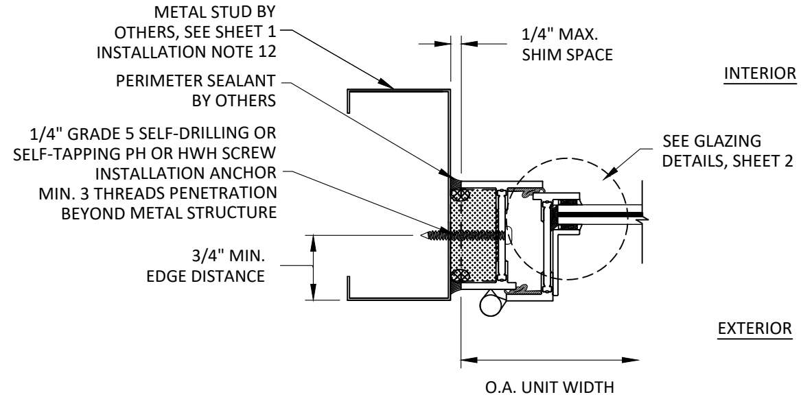
B HORIZONTAL SECTION 10 JAMB- METAL STUD THROUGH FRAME INSTALLATION LONG LEG FRAME
