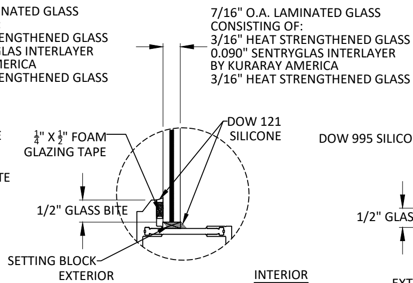
GLAZING DETAIL 6
