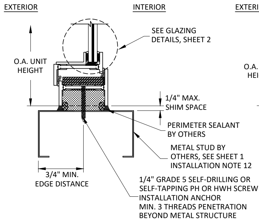
E 7 VERTICAL SECTION SILL - METAL STUD THROUGH FRAME INSTALLATION LONG LEG FRAME
