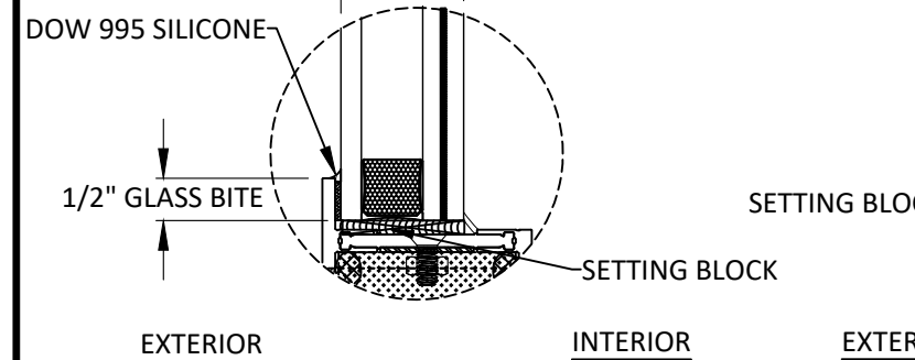
GLAZING DETAIL 1
