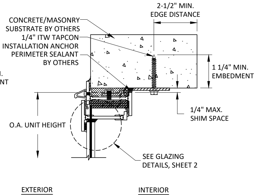
C 6 VERTICAL SECTION HEAD - CONCRETE/MASONRY FLANGE/STRAP INSTALLATION UNEQUAL LEG FRAME
