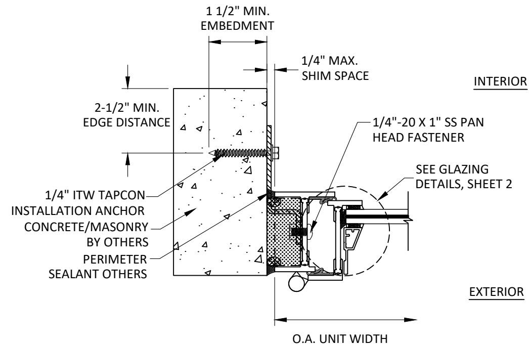
A 9 HORIZONTAL SECTION JAMB- CONCRETE/MASONRY STRAP INSTALLATION LONG LEG FRAME
